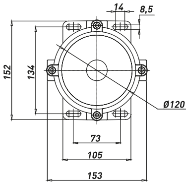
CPSG/CPST/CPSX
