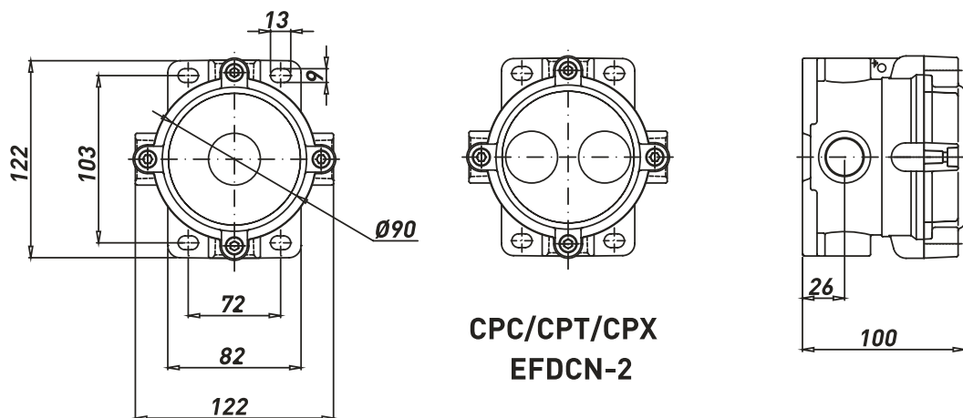
CPC/CPT/CPX EFDCN-1
